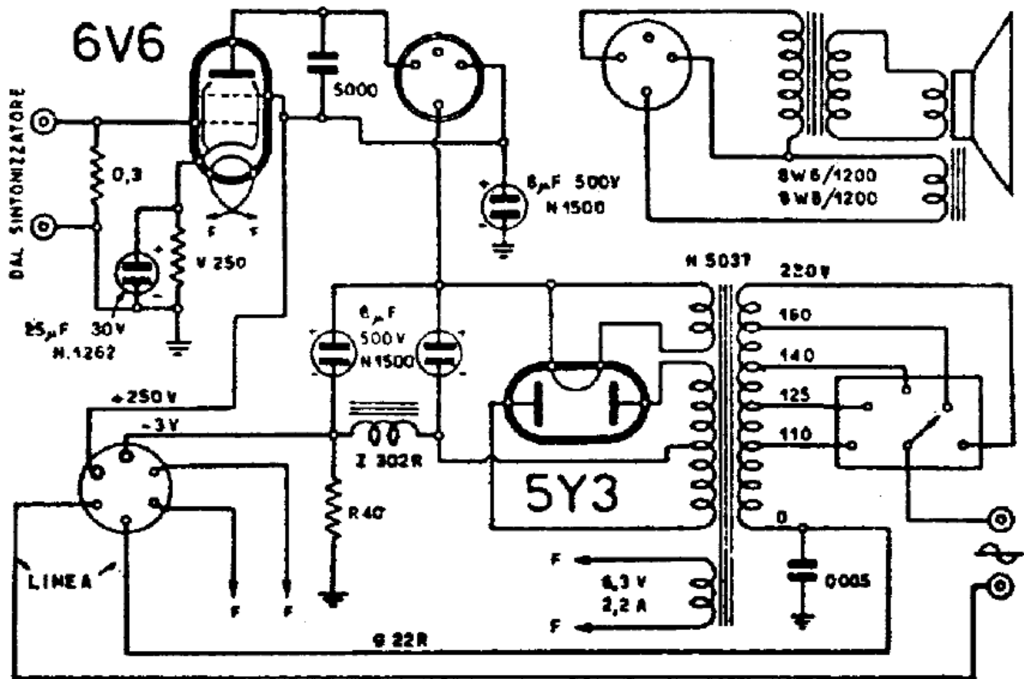
Geloso G22R Power Supply
